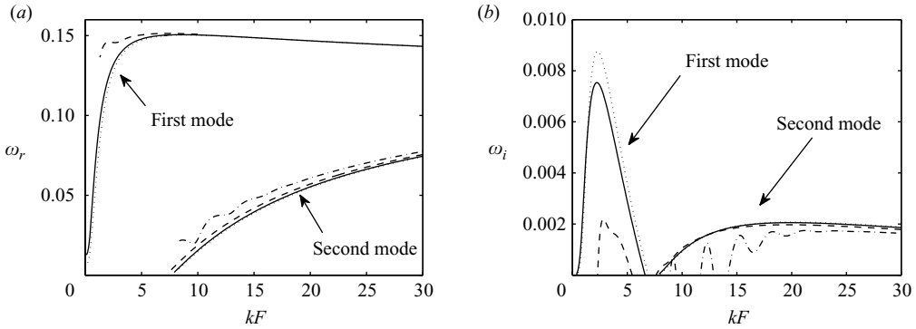
FIGURE 5. Variation of the first two branches with respect to the Froude number in the weakly stratified case for m=1 and Re=\infty . (a) Frequency \omega_r and (b) growth rate \omega_i versus k , for F=0.1 (dotted line), F=1 (solid line), F=2 (dashed line) and F=3 (dash-dotted line).
