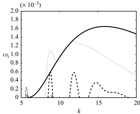
FIGURE 23. Maximum growth rate versus k of the first mode m=2 for Re = \infty . F=0.5 (thick solid line), F=0.75 (dotted line), F=1 (dash line), F=1.5 (solid line)
