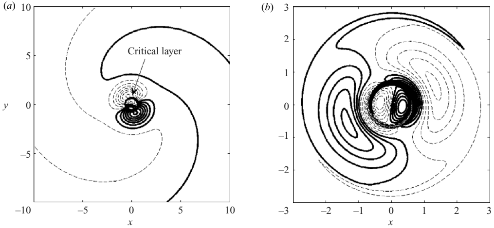
FIGURE 6. (a) Density and (b) vorticity structure of the first helical mode ( m = 1 ) for F = 1.5 , Re = 10^5 , k = 1.6 , \omega = 0.136 + 0.00538i . The critical radius is here r_c \approx 0.68 .
