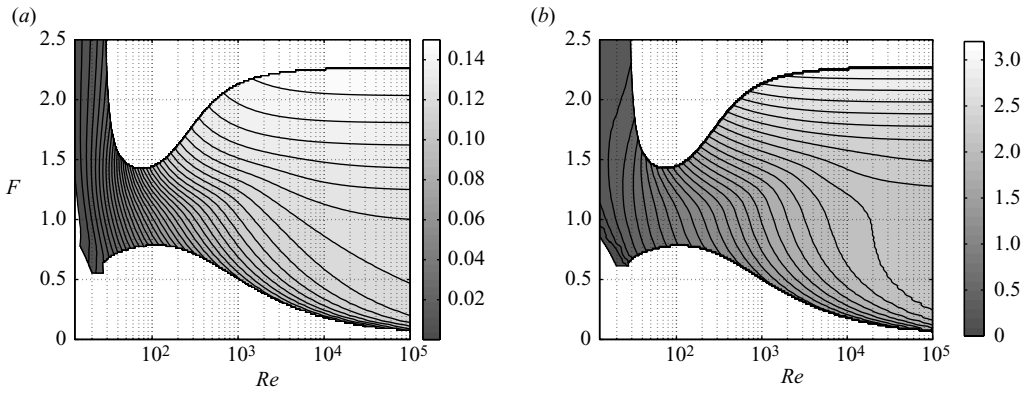
FIGURE 11. Characteristics of the most unstable first helical mode as function of F and Re . (a) Isocontours of the frequency \omega_r ; (b) isocontours of the product kF .
