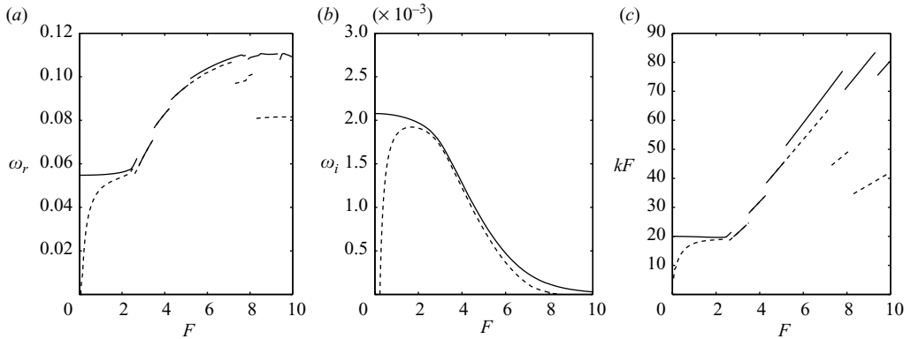
FIGURE 13. Characteristics of the most unstable second helical mode for Re = \infty (solid line) and Re = 10^6 (dashed line) as a function of the Froude number F . (a) Frequency \omega_r ; (b) growth rate \omega_i ; (c) product kF .
