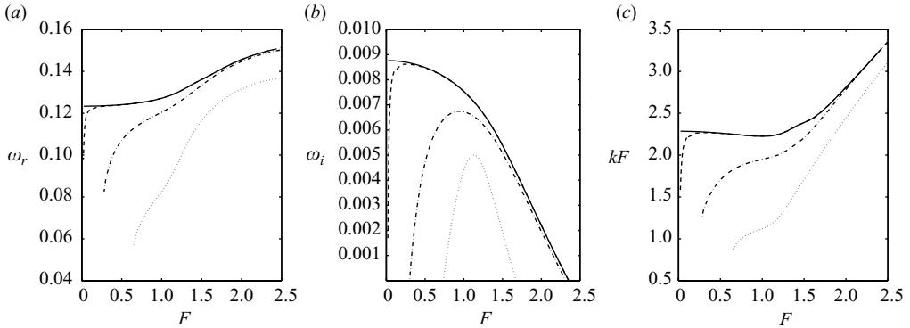
FIGURE 9. Characteristics of the most unstable first helical mode for Re = \infty (solid line), Re = 10^6 (dashed line), Re = 3000 (dash-dotted line), Re = 200 (dotted line) as a function of the Froude number F . (a) Frequency \omega_r ; (b) growth rate \omega_i ; (c) product kF .
