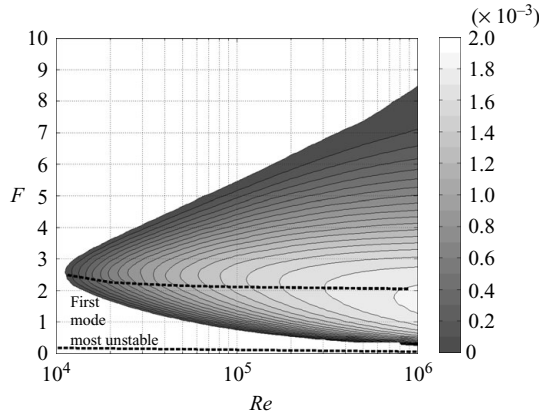
FIGURE 12. Maximum-growth-rate contours of the second helical mode ( m = 1 ) as functions of the base-flow parameters F and Re . The dashed curves delimit the unstable region in which the first helical mode is more unstable.
