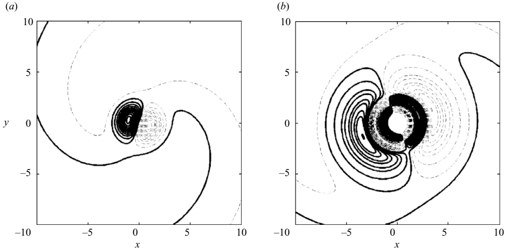
FIGURE 4. Density structure of the first two most unstable helical modes for F = 0.9 and Re = \infty . (a) First mode obtained for k = 2.5 , \omega = 0.126 + i0.0078 ; (b) second mode (first ring mode) obtained for k = 22.1 , \omega = 0.055 + i0.00206 . The solid lines (respectively dashed lines) are the positive (respectively negative) contours.
