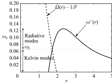
FIGURE 16. Theoretical predictions for the frequency domain of existence of quasi-neutral modes for m=1 and F=4 . The dashed line is the plot of \Omega(r) - 1/F which defines the location of the critical point II; the solid line is the plot of \omega^-(r) which defines the location of the turning points.
