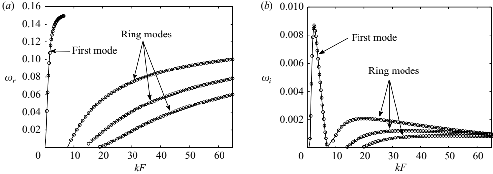
FIGURE 3. (a) Frequency \omega_r and (b) growth rate \omega_i of the first four more unstable modes for Re = \infty , F = 0.9 . The symbols represent our results with Np = 150 , H = 3 , \theta = \pi/10 . The lines represent results obtained by the shooting method of Le Dizès & Billant (2009). Only the unstable modes have been plotted.
