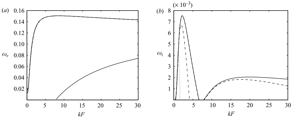
FIGURE 7. Variation of the first two branches with respect to the Reynolds number for m = 1 , F = 1 . (a) Frequency \omega_r and (b) growth rate \omega_i versus kF for Re = \infty (solid line), Re = 10^6 (dashed line), Re = 3000 (dash-dotted line), Re = 200 (dotted line).
