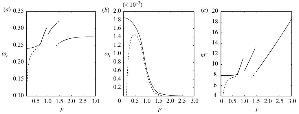
FIGURE 22. Characteristics of the most unstable mode m = 2 as a function of the Froude number for Re = \infty (solid line), Re = 10^6 (dashed line). (a) Frequency \omega_r ; (b) growth rate \omega_i ; (c) product kF .
