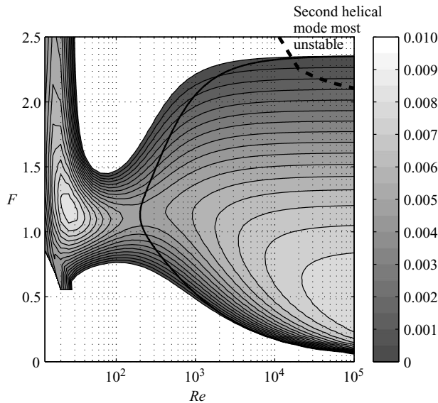
FIGURE 8. Maximum-growth-rate contours (maximum over k ) of the first helical mode ( m = 1 ) as a function of the base-flow parameters F and Re . The dashed curve delimits the unstable region in which the first helical mode is not the most unstable mode. The thick solid curve delimits the region in which the growth rate is larger than 1/Re . To the left of this curve, the viscous diffusion of the base flow is expected to affect the results.
