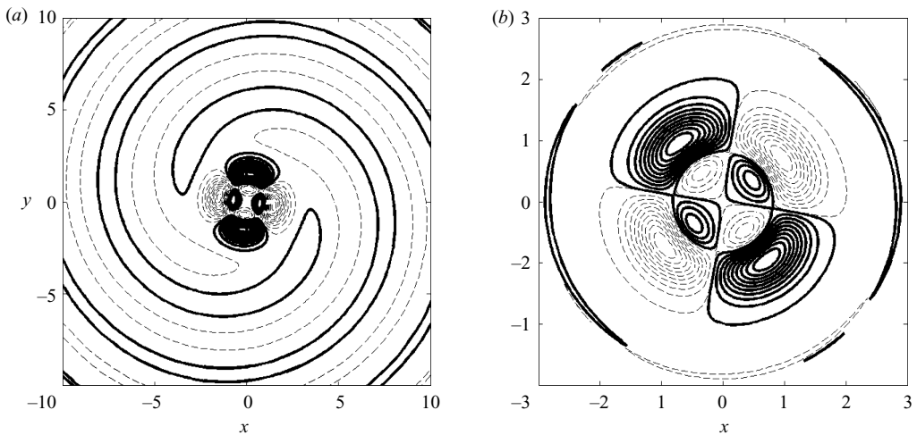
FIGURE 20. Structure of the eigenmode m=2 , k=19.8 and \omega=0.244 + i0.00173 for F=0.4 and Re = \infty . (a) Density contours; (b) axial vorticity contours.
