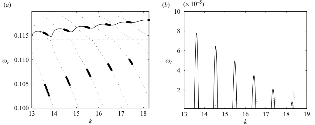
FIGURE 15. Dispersion relation of the helical modes for Re = \infty and F = 8 . (a) Frequency \omega_r and (b) growth rate \omega_i . The modes shown in (a) are damped except in the thick part of the curve where the growth rate is given in (b). The solid and dotted lines correspond to radiative and Kelvin modes respectively. Modes with a growth rate smaller than -3 \times 10^{-2} have not been plotted in (a). The horizontal dashed line in (a) is the theoretical prediction of maximum resonance.
