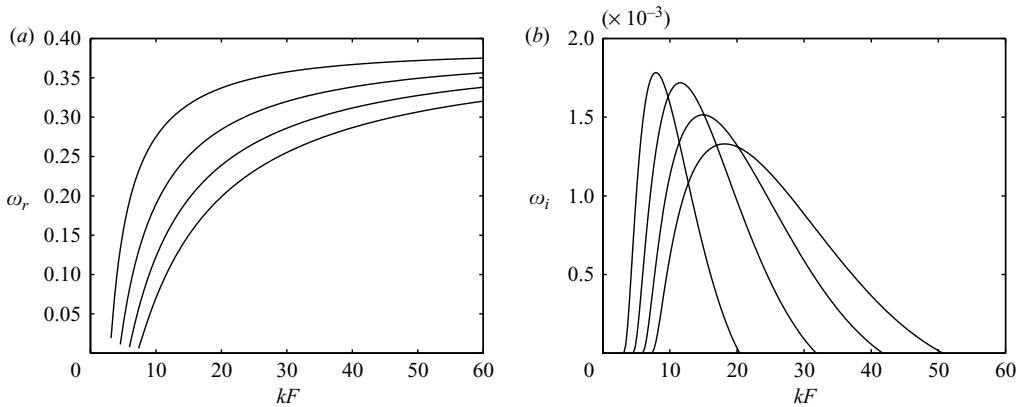
FIGURE 18. (a) Frequency \omega_r and (b) growth rate \omega_i for m = 2 , Re = \infty and F = 0.3
