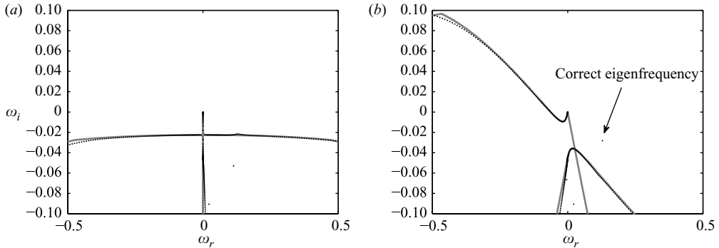
FIGURE 2. Close view of the numerical spectrum (dots) and theoretical continuous spectrum (solid grey lines) near a correct damped eigenvalue (indicated by the arrow) for the parameters of figure 1 and Np = 400 and H = 12 . (a) Real path \theta = 0 ; (b) complex path \theta = \pi/10 .
