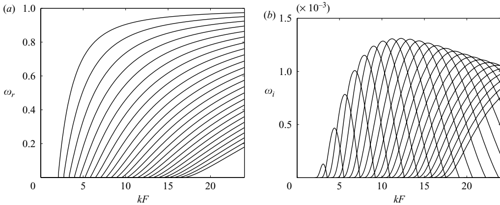
FIGURE 19. (a) Frequency \omega_r and (b) growth rate \omega_i for m=3 , Re = \infty and F=0.2
