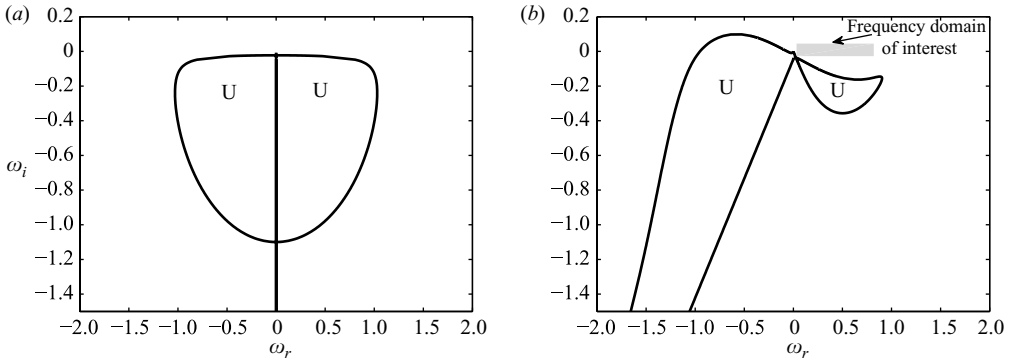
FIGURE 1. Continuous spectrum (solid lines) and ‘unphysical’ domain (indicated by the letter ‘U’) for Re=200 , F=0.9 , k=3 . (a) Real path \theta=0 ; (b) complex path \theta=\pi/10 .
