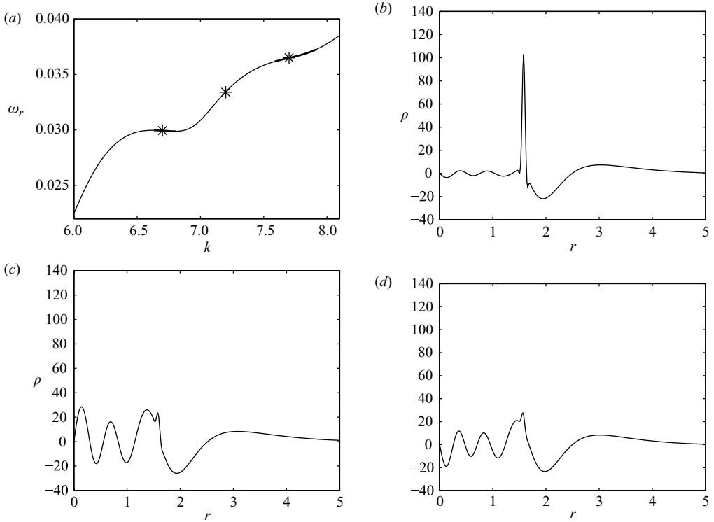
FIGURE 17. Structure of the resonant/non-resonant modes for m = 1 , F = 3 , Re = 10^5 . (a) Frequency of the third helical mode (second ring mode). The thick line is the unstable domain. The radial profile of the eigenmode density at the crosses is given in (b)–(d): (b) kF = 7.2 (stable); (c) kF = 6.7 (unstable); (d) kF = 7.7 (unstable).
