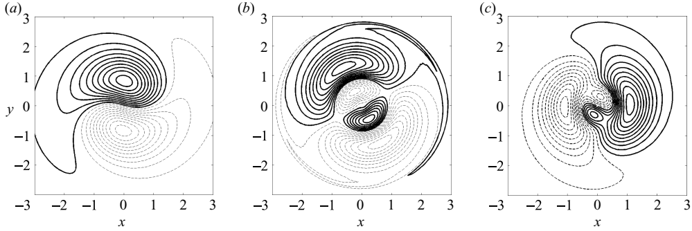
FIGURE 10. Axial vorticity contours in the plane of the first helical eigenmode for F = 1.15 and (a) Re = 26 , k = 0.38 , \omega = 0.0195 + i0.00878 , (b) Re = \infty , k = 1.95 , \omega = 0.129 + i0.00706 , (c) Re = 80 , k = 0.8 , \omega = 0.0682 + i0.00566 .
