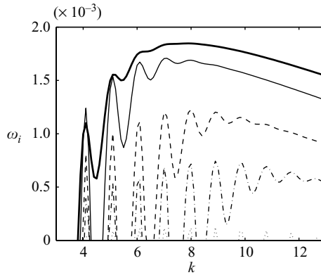
FIGURE 14. Maximum growth rate versus k of the second helical mode for Re = \infty : F = 2.5 (thick solid line), F = 3 (solid line), F = 4 (dashed line), F = 5 (dash-dotted line), F = 7 (dotted line).
